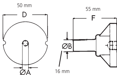
1/2" thread, 12.7 mm DEEP - 2 HOLES B162-2Q With 4/0 AWG Stud (120 mm 2 )
