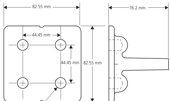
1/2" thread, 12.7 mm DEEP - 4 HOLES B164-2Q With 4/0 AWG Stud (120 mm 2 )
