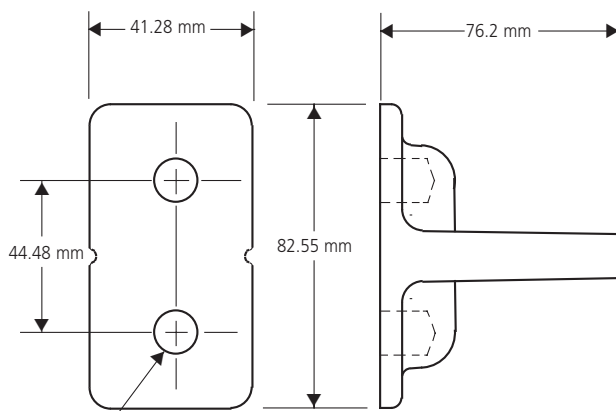
1/2" thread, 12.7 mm DEEP - 2 HOLES B162-2Q With 4/0 AWG Stud (120 mm 2 )
